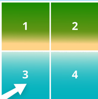
Gradient wind:
